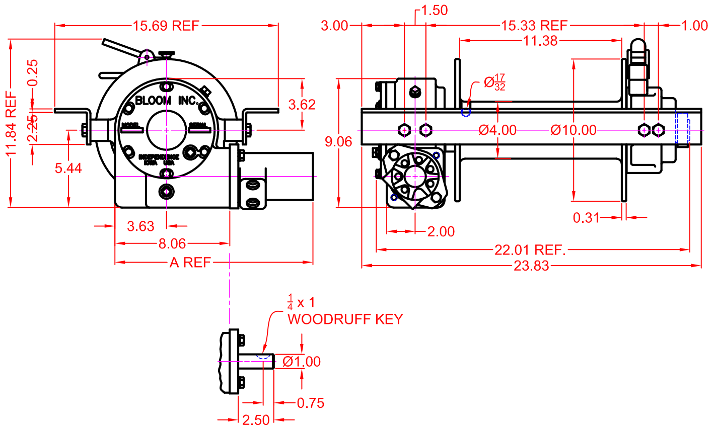
INPUT SHAFT MODEL
