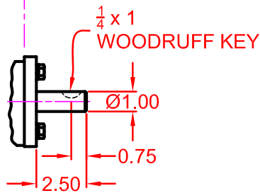
INPUT SHAFT MODEL
